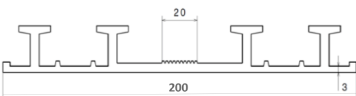
CL-Waterstop PV28200
