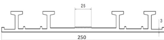
CL-Waterstop PV29250
