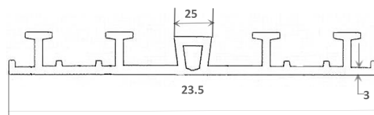
CL-Waterstop PV25250
