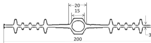
CL-Waterstop PV52200
