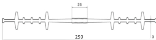
CL-Waterstop PV57250
