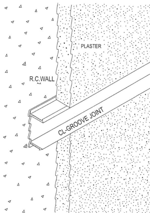
Three dimensional view of the CL-GROOVE JOINT being installed with plaster rendered onto the wall.
