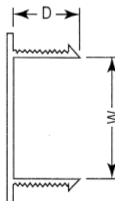
Cross sectional view of CL-GROOVE JOINT
